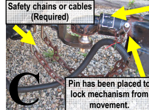
Locking mechanism has been moved forward to lock trailer hitch to ball on vehicle.
